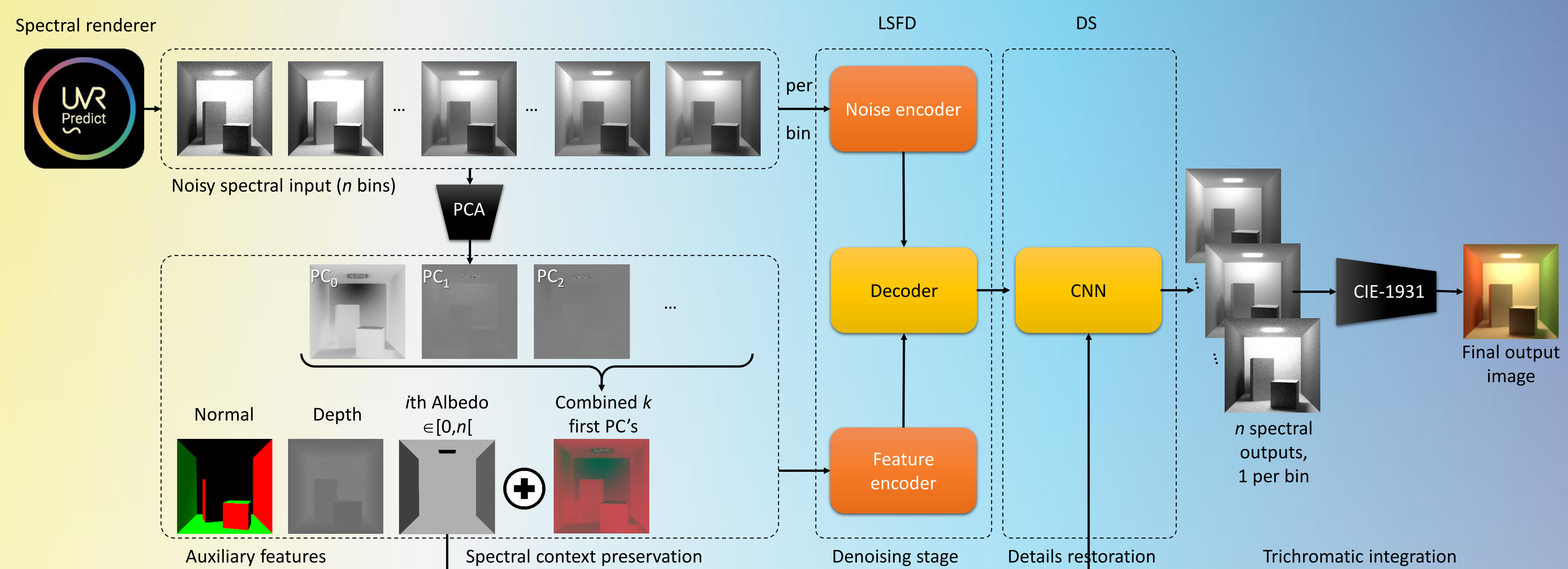
Figure 2: Overview of our spectral denoiser
